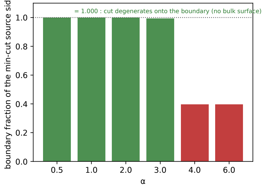
(b) for \alpha \leq d there is no bulk min-cut surface
