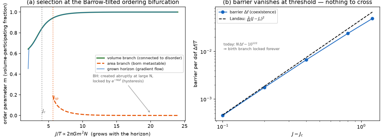
FIG. 4. Selection at the ordering bifurcation. (a) With the Barrow tilt, the minimum continuously connected to the disordered state is the volume branch (green); the area branch (orange, dashed) is born metastable only at the spinodal J_{\text{sp}} > J_c and is never occupied by the grown horizon, whose gradient-flow trajectory (blue) tracks the volume branch with no discontinuity. A black hole, created abruptly at large N , starts on the area branch and is locked there by exact long-range hysteresis. (b) The barrier vanishes quadratically at threshold — Landau’s 3(J - J_c)^2/64 — so the grown horizon crossed the bifurcation when there was nothing to cross; today’s N \cdot \Delta f \sim 10^{122} locks the birth branch forever.
