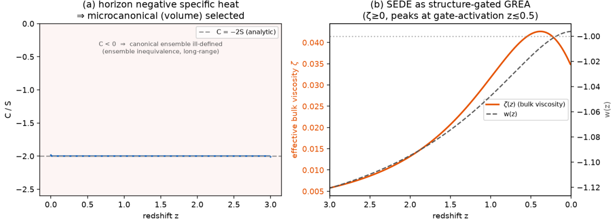
FIG. 2. Two consequences drawn from the new literature. (a) The de Sitter horizon has negative specific heat ( C = -2S ); with gravity strongly long-range this makes the ensembles inequivalent and the canonical (area-law) accounting ill-defined, selecting the microcanonical (volume) branch (§IV). (b) SEDE’s structure-driven entropy production maps to a positive (second-law) effective bulk viscosity \zeta(z) that peaks at the gate-activation epoch ( z < \sim 0.5 ; it tracks d \ln f_{\text{sat}}/d \ln a , not the z \approx 2 star-formation peak), casting SEDE as a structure-gated member of the GREA/entropic-dark-energy family; w(z) crosses -1 at the viscous–dilution balance.
