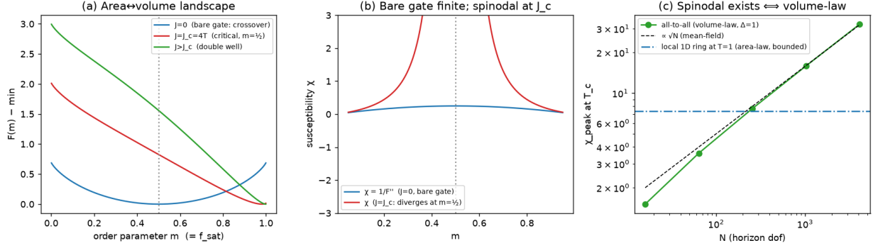
FIG. 3. The two-phase horizon free energy. (a) Smooth crossover for the bare gate ( J = 0 ); a spinodal develops only for J \geq J_c . (b) The bare-gate susceptibility is finite; it diverges at the spinodal. (c) The cooperative coupling J = \lambda_{\max}(W_{\text{grav}}) is the gravitational binding itself: all-to-all (volume-law) connectivity gives \chi_{\text{peak}} \propto \sqrt{N} (so J/J_c \sim N , far above threshold), while local (area-law) connectivity is bounded. Gravity thus makes the well bistable — but deeply so today, which is why selection happens at the birth bifurcation (result iii, Fig. 4) rather than by barrier crossing (the horizon’s membrane hydrodynamics, result iv, is a separate matter). The landscape variable here is the order parameter m of (ii) — the fraction of horizon bonds on the bulk side of the min-cut — and not the cosmological gate f_{\text{sat}} ; the two are distinct coordinates and must not be read against each other (see the caution below).
