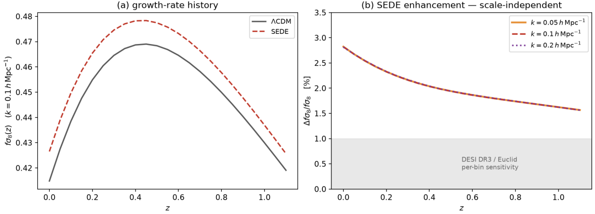
Figure 3. The growth prediction. (a) f\sigma_8(z) at k = 0.1 \text{ h/Mpc} for \Lambda\text{CDM} and SEDE at the shared best-fit cosmology. (b) The fractional SEDE enhancement at k = 0.05, 0.1 and 0.2 \text{ h/Mpc} — the three curves lie on top of one another, which is the point: the enhancement is scale-independent through the RSD range, entering the DESI DR3/Euclid sensitivity band. Underlying data: src/fsigma8_prediction.json , regenerated by src/sims/sede_fsigma8_isw_finitek.py .
