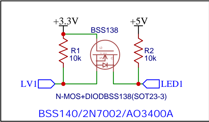
Logic Level Shifter
