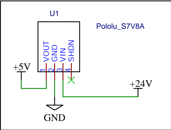
24V -> 5V
