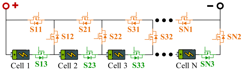
Fig. 6. Schematic diagram of a series-connected three-switch topology proposed in [26].
