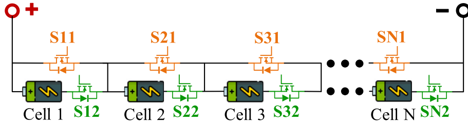
Fig. 4. Schematic diagram of series-connected battery topology introduced in [15].
