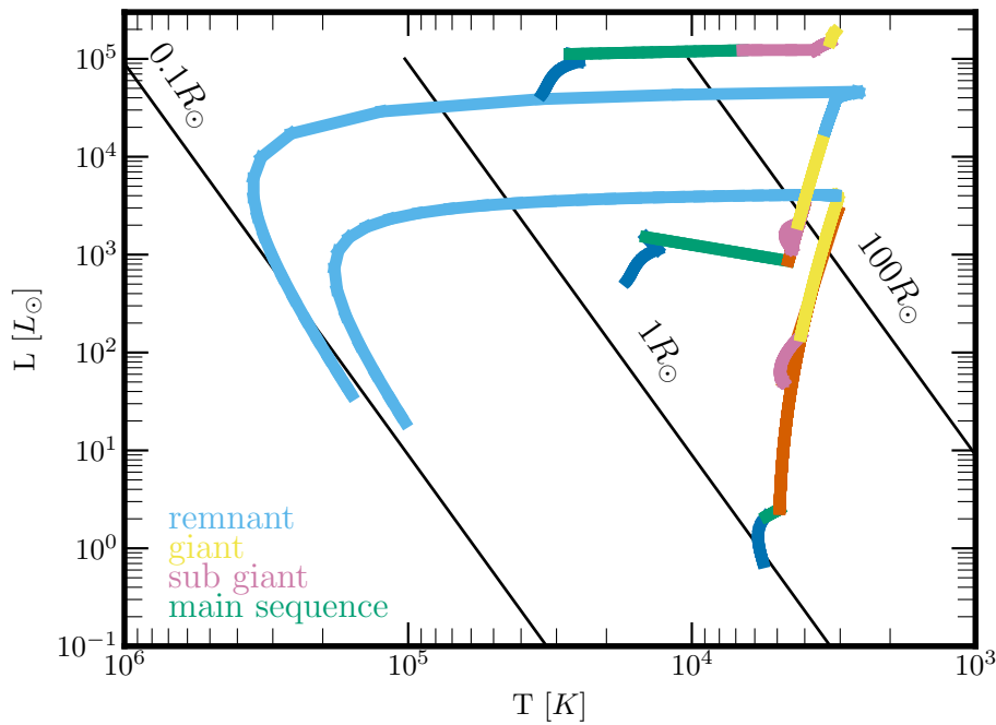
Figure 5.3: Hertzsprung–Russell diagrams (luminosity versus temperature) for three stars of masses 1 M_{\odot} (bottom set curves), 5 M_{\odot} , and 20 M_{\odot} (top curves), from the zero-age main sequence to the moments they turn into compact remnants. The colored text in the bottom left identifies the evolutionary stage of the star along its track (with the caveat that a star at the tip of the asymptotic giant branch should probably not be identified as a remnant). The black diagonal lines indicate the run of luminosity and temperature for blackbodies with radii 0.01 R_{\odot} (left), 1 R_{\odot} , and 100 R_{\odot} (rightmost line). The figure was made using the script amuse.examples.plot_stellar_evolution_track .
