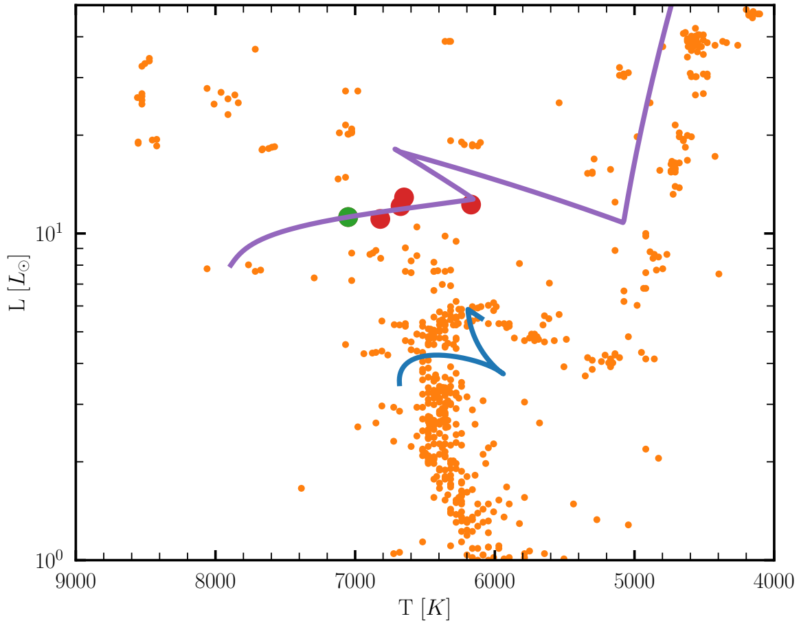
Figure 5.10: Hertzsprung–Russell diagram for the star cluster M67. The data are from http://webda.physics.muni.cz/ (Eggen & Sandage, 1964). The red (the stars S984, S975, S997, and S2204) and green (S1082) bullets are the blue stragglers listed in Table 5.3. The other bullet points (orange) are the M67 stars. Two lines indicate the evolutionary track for a star near the turn-off of 1.4 M_{\odot} (blue) and 1.7 M_{\odot} (purple), both at twice the solar metallicity ( Z = 0.02 ). This figure was generated using the script amuse.examples.plot_M67withBSS_tracks . It should take 5–10 s to run on a laptop.
