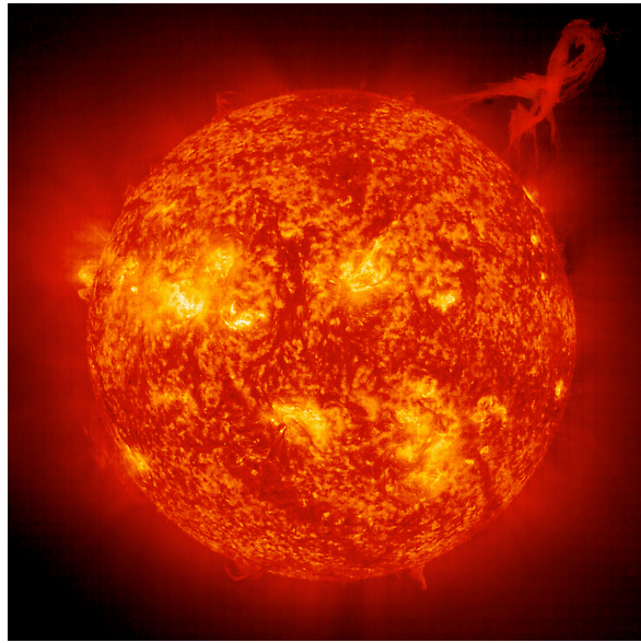
Figure 5.5: Surface image of the Sun (image from the SOHO mission at EIT 304 Å on 1999 September 14). The light and dark orange patches (as opposed to the yellow areas, which are regions of solar activity) show granulation, the result of temperature variations due to convection just below the surface. Image from ESA/NASA/SOHO/EIT Courtesy of SOHO/EIT consortium. SOHO is a project of international cooperation between ESA and NASA.
