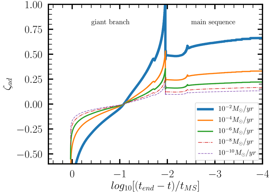
Figure 5.9: Response of an M = 1 M_{\odot} star to mass loss, expressed as a function of time (relative to the main sequence lifetime). We performed the calculation for mass-loss rates dm/dt = 10^{-2} M_{\odot}/\text{yr} (top curve), dm/dt = 10^{-4} M_{\odot}/\text{yr} , 10^{-6} M_{\odot}/\text{yr} , 10^{-8} M_{\odot}/\text{yr} , and 10^{-10} M_{\odot}/\text{yr} (bottom curve). The figure was created using a script based on amuse.examples.stellar.massloss_response . The calculation took several hours on a laptop, so we include the data file ( Zeta_M1MSun_for_various_dmdt.data in the data directory) for a 1 M_{\odot} star and plot this using the amuse.examples.plot_stellar_massloss_response module.
