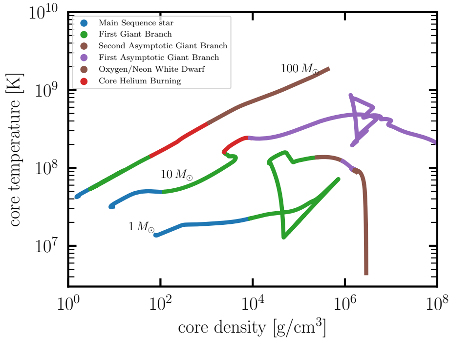
Figure 5.6: Central temperature as a function of core density for a 1 M_{\odot} (bottom), a 10 M_{\odot} (middle), and a 100 M_{\odot} star (top) of solar metallicity. The colors identify various evolutionary phases (see legend), starting with the main sequence at the lower left to giants and white dwarfs to the right. The code to produce this plot can be found in amuse.examples.stellar.calculate_core_temperature_density (see Code example 5.1). To plot the results it may be more practical to use the pre-calculated data in the simple plotting script amuse.examples.plot_core_temperature_density , because the Henyey stellar evolution code Mesa (see Table 5.1) used to generate this figure takes a few hours for each single star. In particular the 1 M_{\odot} star tends to be slow along the asymptotic giant branch just before the green part of the curve; magnifying this part of the evolution will reveal interesting sinusoidal variations in the core density and core temperature of the star.
