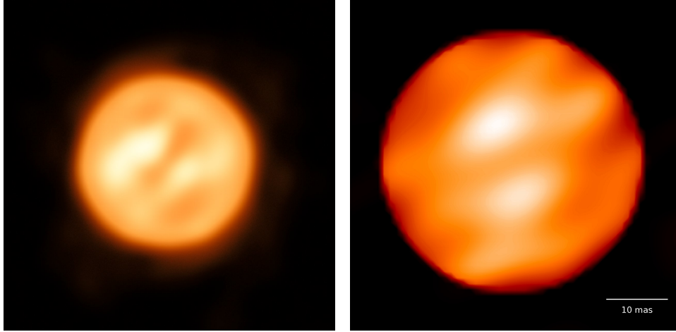
Figure 5.1: Stars are finite objects with structure on their surface, as demonstrated here with the observations of Antares (left, image with the ESA VLTI; reprinted with permission from Ohnaka et al. , 2017 ) and Betelgeuse (right, image by Observatoire de Paris; reprinted with permission from Haubois et al. , 2009 ). Both stars are similar in size—about 4.1–5.5 au ( Dolan et al. , 2016 ). For comparison, we also show an image of the nearest white dwarf, Sirius B, with a size of 0.008 R_{\odot} , next to the two red giants.
