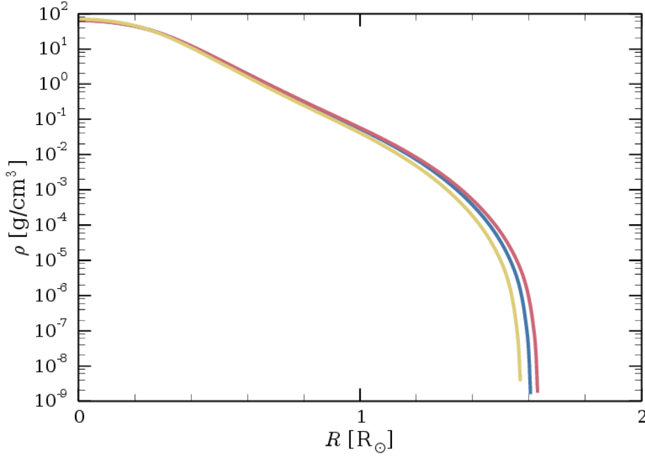
Figure 5.7: Density profile of a star on the zero-age main sequence. All three curves are for a single 2M_{\odot} star. Two curves are calculated using the stellar structure and evolution codes EVTWIN (blue curve) and Mesa (red). The yellow curve is generated from a merger of two 1M_{\odot} stars, which are combined conservatively using MMAMS for constructing a 2M_{\odot} in dynamical equilibrium, whose structure is then calculated using Mesa . The merger calculation is performed using the script in Code example 5.5. The script to generate this figure can be found in amuse.examples.stellar.merger_stellar_density_profile .
