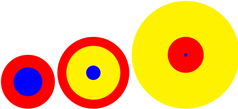
Figure 5.2: Schematic structure of a low-mass star (left), an intermediate-mass star (middle) and a high-mass star (right). They are not to scale, but the various colored regions in the stellar interior indicate the nuclear-burning region (blue), the convective zone (red), and the radiation-dominated region (yellow).
