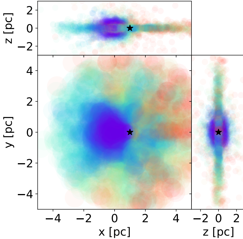
Figure 7.3: Top, and sideview of the gas distribution around the 100 L_{\odot} star from the calculation presented in Figure 7.2. The bump to the left of the star shields the disk from radiation, and remains cold. The temperature distribution in the disk is radially structured, depending on clumpiness in the particle distribution in the disk. The color coding according to the colorbar in Figure 7.2. amuse.examples.rad_minimal .
