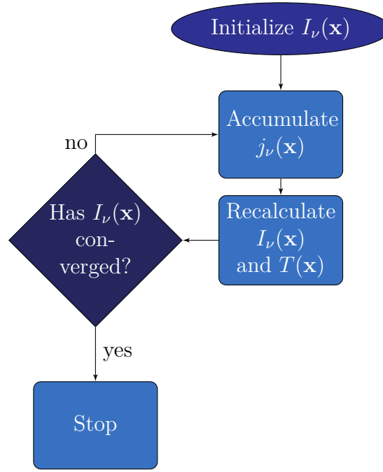
Figure 7.1: Workflow for a radiative transfer code.
