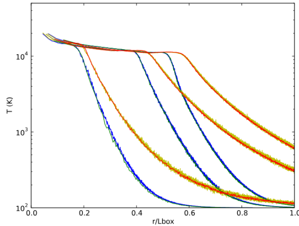
Figure 7.5: Expansion of an ionization front in an initially homogeneous medium (see test #5 of Iliev et al. (2009)). We show here the temperature structure as a function of distance (normalized to the box size L_{\text{box}} ) after 10, 30, and 200 Myr. The source has a ionizing luminosity L = 5 \times 10^{48} \text{photons s}^{-1} . Calculations are performed using Fi with SimpleX (blue curve), Gadget2 with SimpleX (green), Fi with SPHray (yellow), and Gadget2 with SPHray (red). A more extensive version of this test can be found in Pelupessy et al. (2013), see their Fig.22. Using script amuse.examples.iliev_test5 , this figure can be generated in about 10 minutes on a fast workstation.
