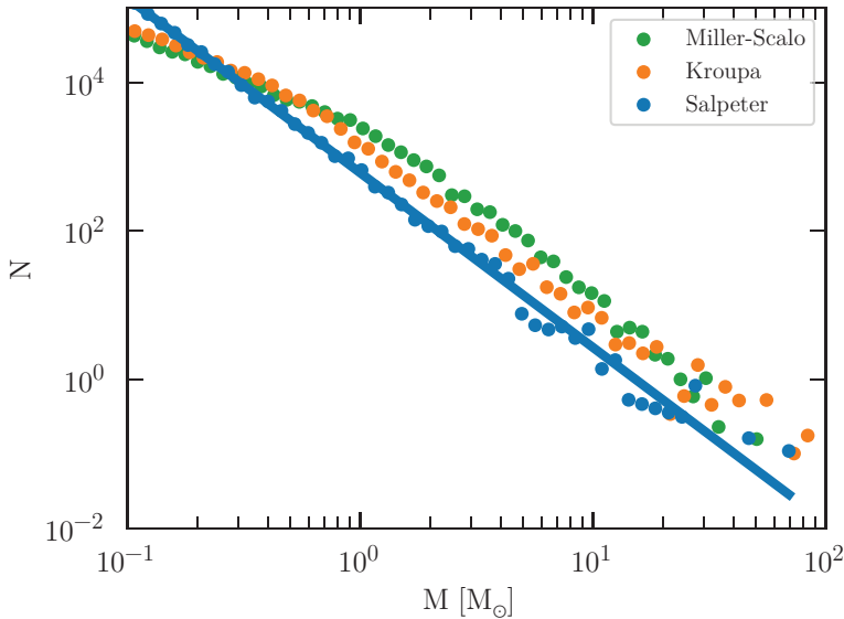
Figure 3.3. Initial mass function for 10^4 stars between 0.1 M_\odot and 100 M_\odot . The Salpeter mass function is overplotted with an analytic power law with a slope of -2.35 (blue). Two other frequently used mass functions are shown in green and orange. The latter two are described by Miller & Scalo (1979) (in green) and Kroupa (2001) (orange). An example of how this is plotted is presented in Code example 3.5. The script to generate this figure can be found in amuse.examples.salpeter . The script to plot these curves is presented in Code example 3.5.
