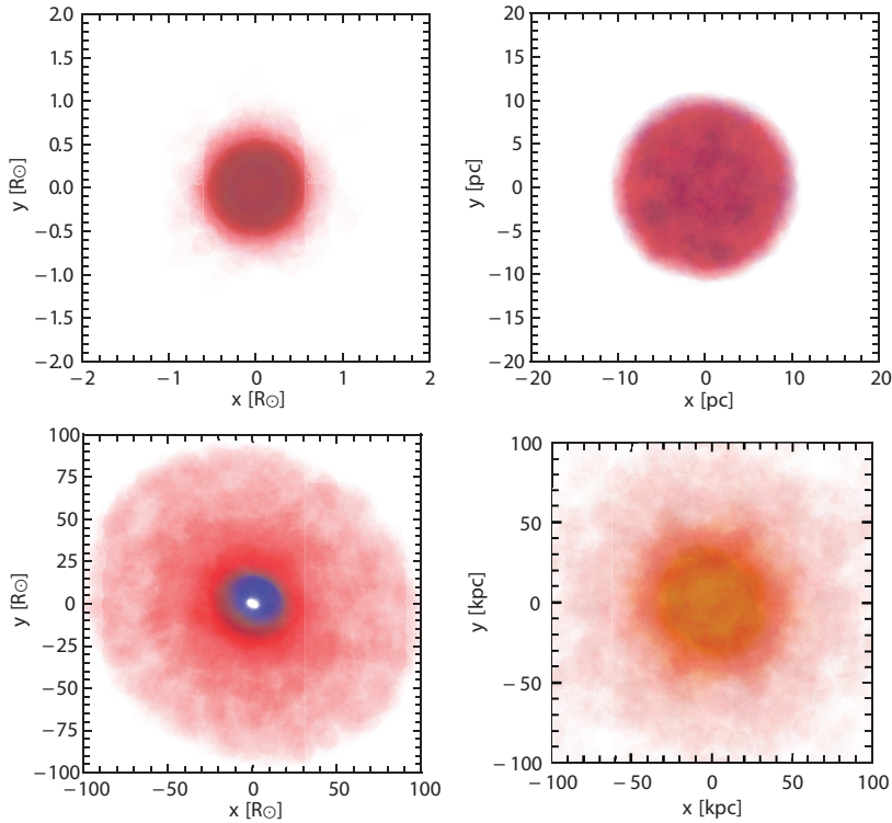
Figure 3.2. Some initial particle distributions for SPH codes. The top-row left panel shows a two solar mass star, the right a homogeneous spherical distribution with a turbulent velocity field, as is often used in simulations of molecular clouds. Particles are colored by their internal energy, from red ( 0.048 \text{ (km s}^{-1})^2 ) to blue ( 1.82 \text{ (km s}^{-1})^2 ). The bottom row shows a slightly tilted circumstellar disk with a total mass of 0.1% of the star's mass (left), and a 10^{10} M_{\odot} galaxy model. The script to generate this figure can be found in amuse.examples.plot_hydro_density_distributions .
