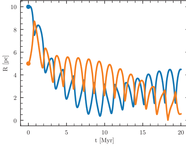
Figure 9.4. Time evolution of Galactocentric distance R of two massive compact objects of 50\,000\,M_{\odot} each from a distance of 10 pc (blue) and 5 pc (orange). Both curves were integrated using a bridge between ph4 for integrating the black holes and a background potential with dynamical friction using \ln(\Lambda) = 3.7 . The sinusoidal variations along the curves are the result of the two black holes not being in a perfect circular orbit. The interference between the two black holes is a consequence of their mutual gravitational interactions. The source code takes a few seconds to run and can be found at amuse.examples.imbhs_with_friction
