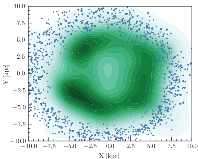
Figure 9.11. Distribution of the Solar siblings (blue bullets) in the Milky Way (green shaded contours). We cut out the central 2 kpc from the Galaxy to keep contrast in the disk. The Sun in this simulation could be anywhere where you see a blue bullet point. The simulation was performed using the script amuse.examples.solar_cluster_in_live_galaxy ; the figure was made with amuse.examples.plot_solar_cluster_in_live_galaxy .
