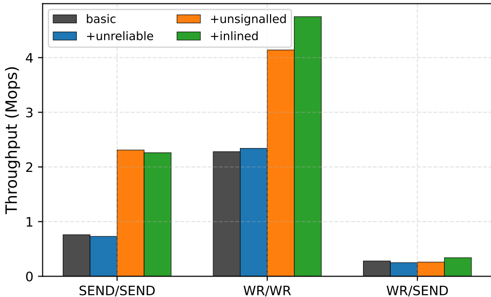
Figure 5: Throughput of ECHOs with 32 byte messages
