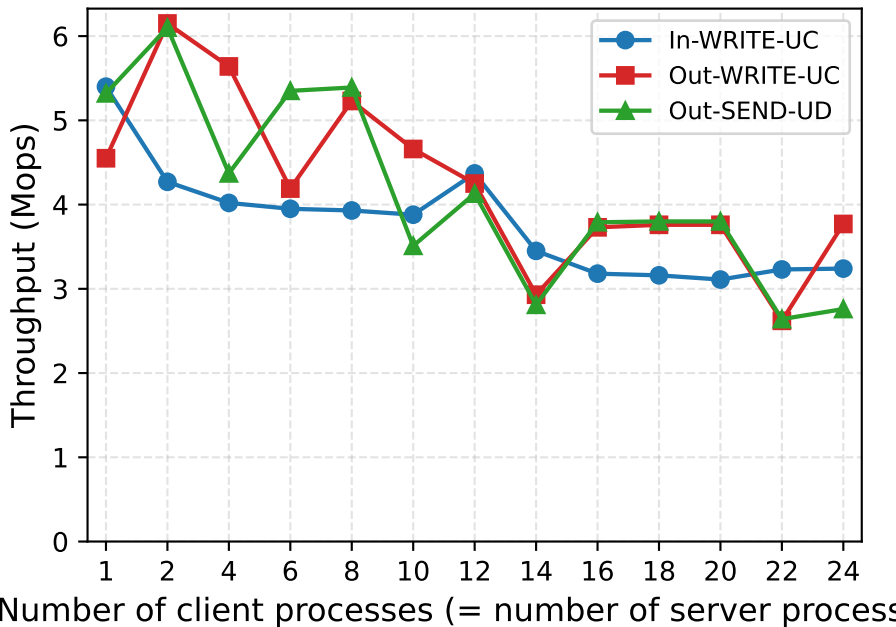
Figure 6: UD vs UC for all-to-all (32 byte payloads)
