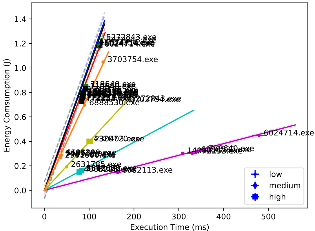
Outliers detected
