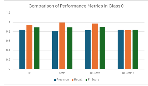
Fig. 6. Comparison of Performance Metrics in Class 0
