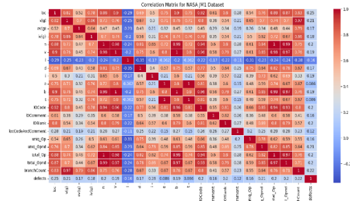
Fig. 3. Correlation Matrix of JM1 Dataset
