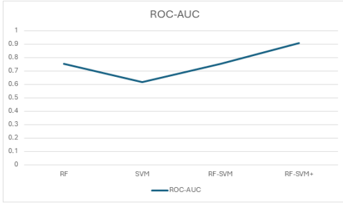
Fig. 9. ROC-AUC Comparison of Classification Models
