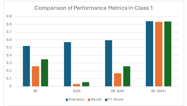
Fig. 7. Comparison of Performance Metrics in Class 1
