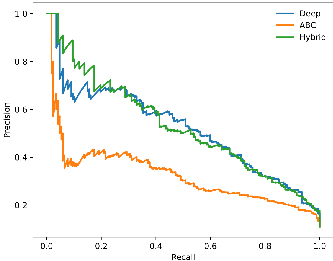
HAM10000 test precision-recall
