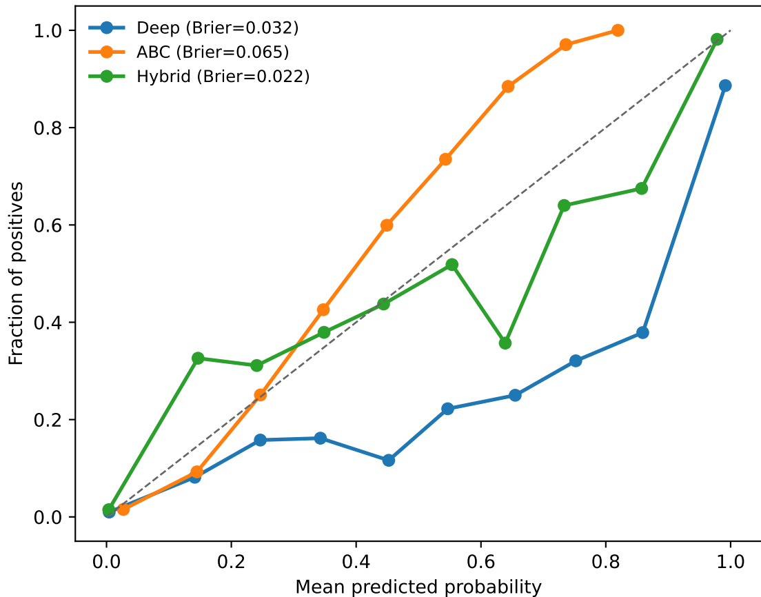
ISIC Task 3-label calibration
