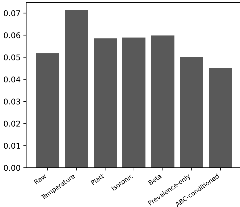
Integrated NB
