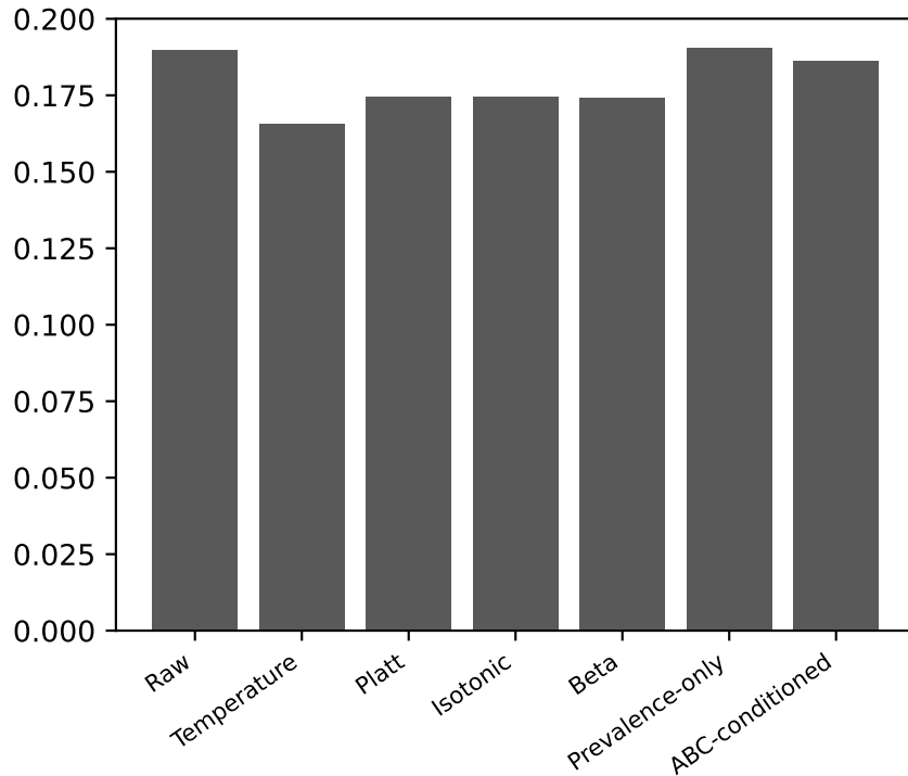
Brier score
