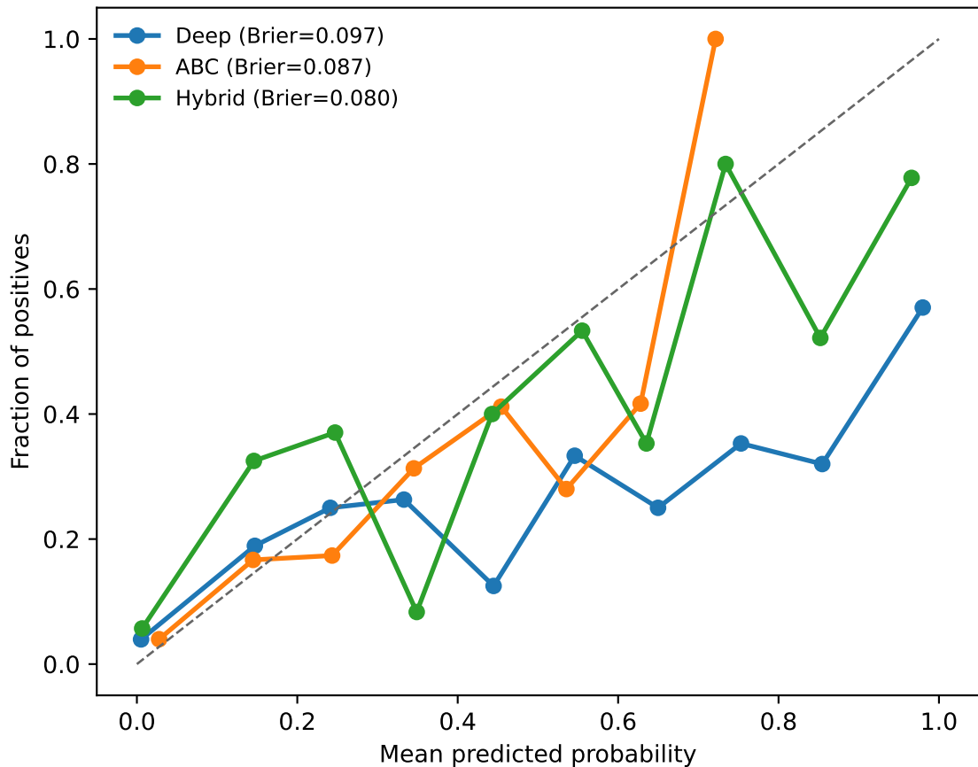
HAM10000 test calibration
