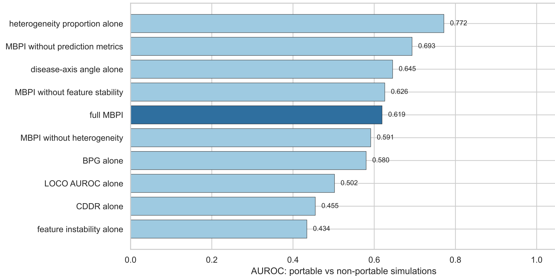
Ablation Benchmark
