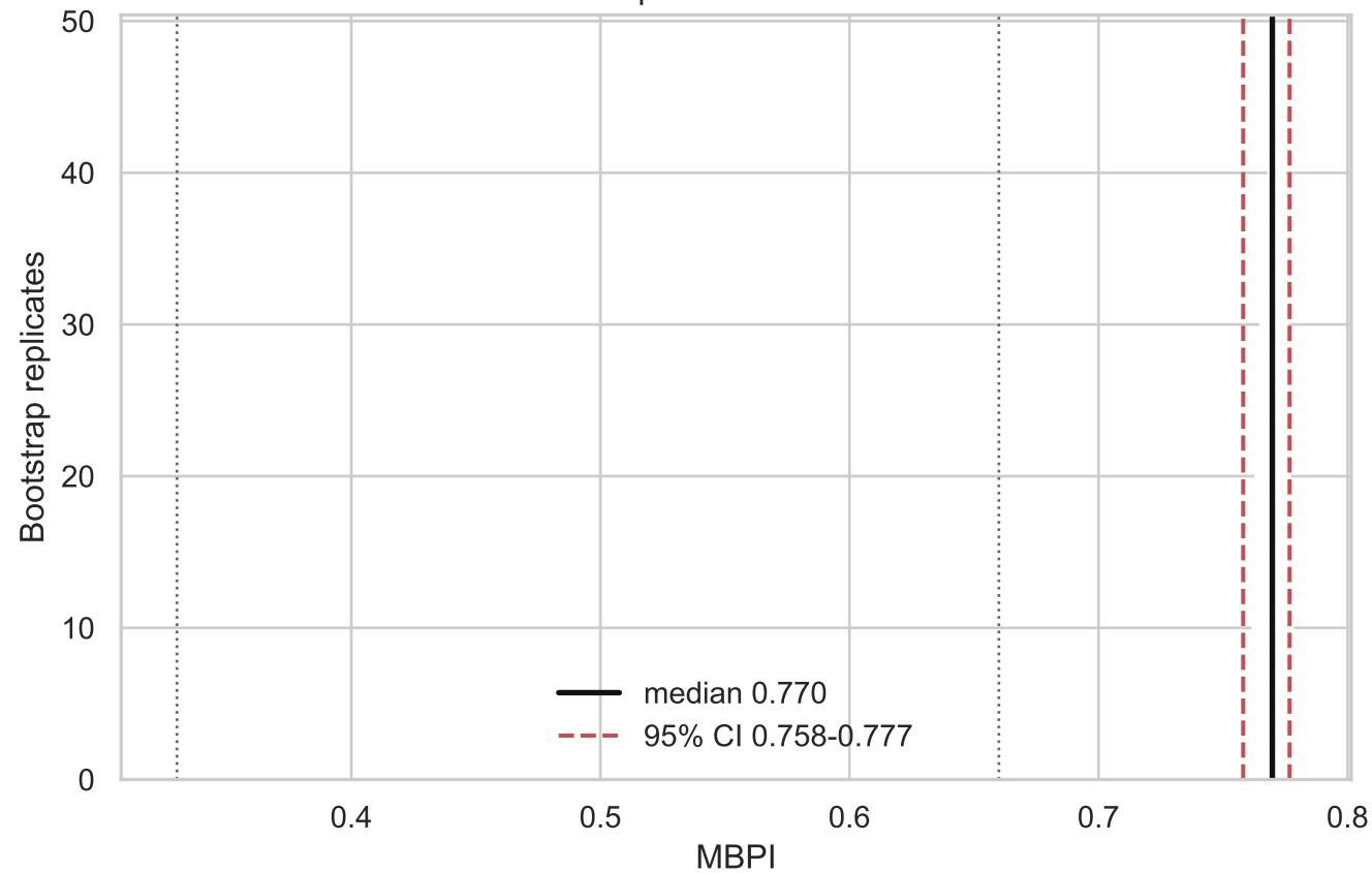
Bootstrap Distribution of MBPI
