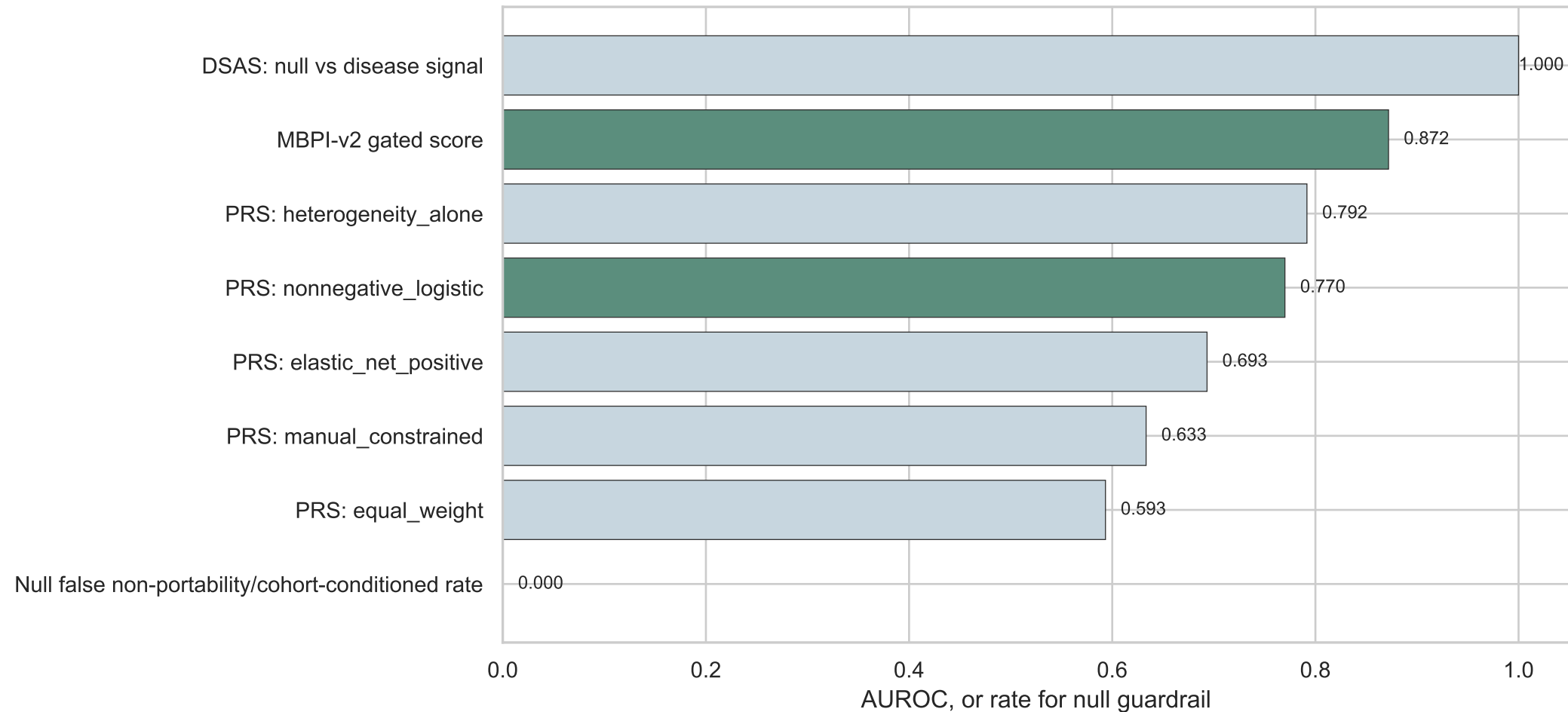
Second Validation MBPI-v2 Ablation
