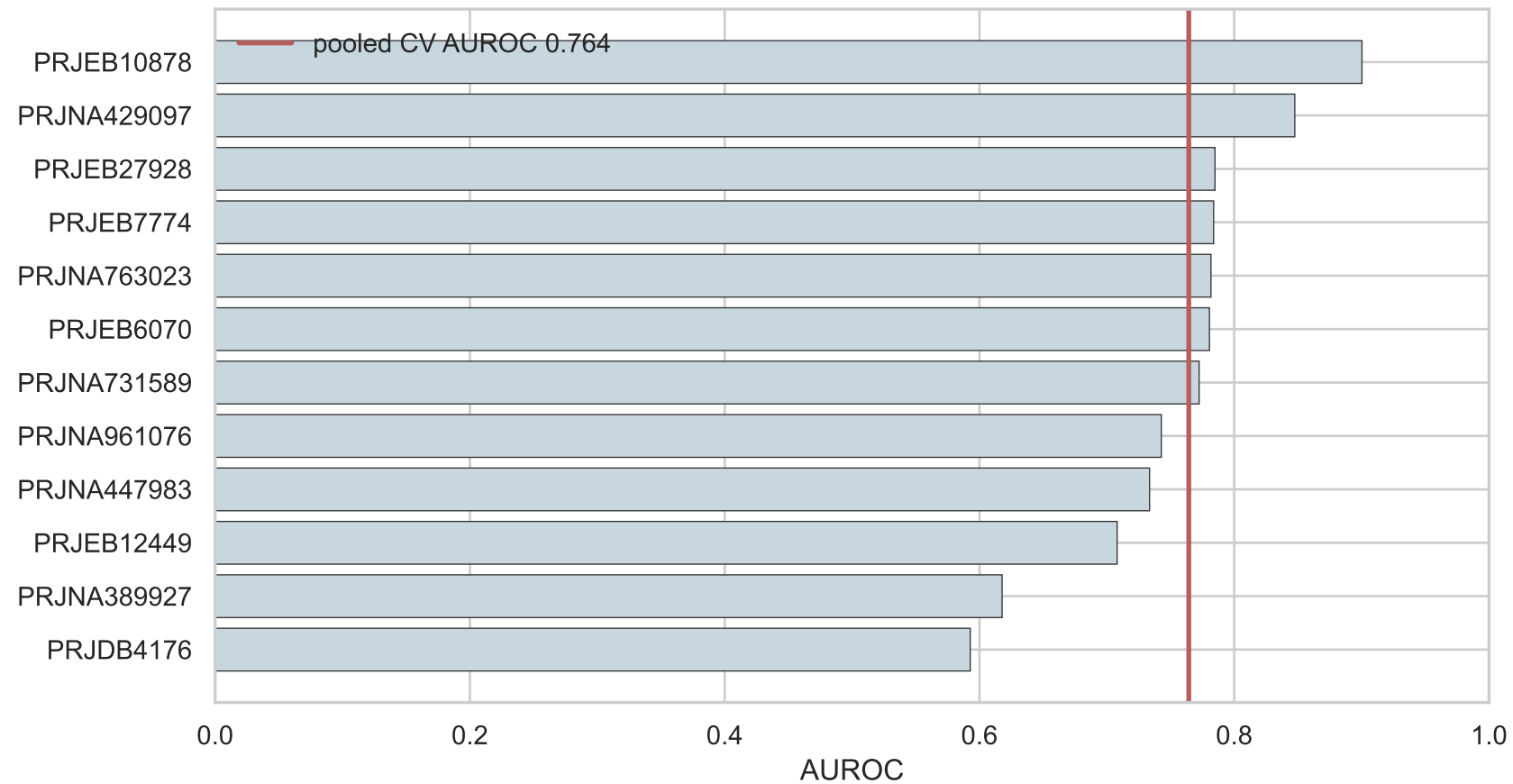
Second Validation Pooled vs LOCO AUROC
