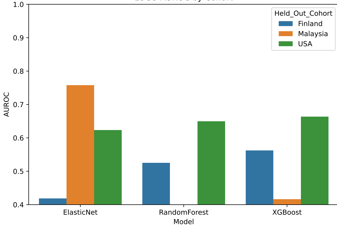
LOCO AUROC by Cohort
