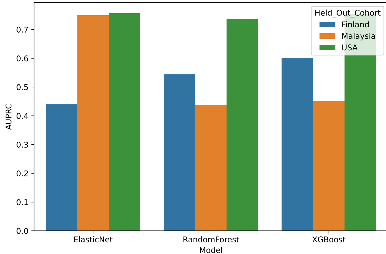
LOCO AUPRC by Cohort
