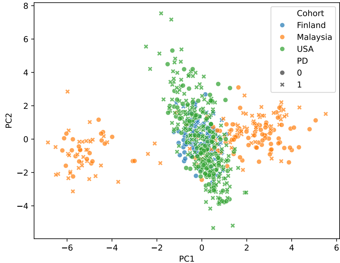
PCA Global Residualized CLR
