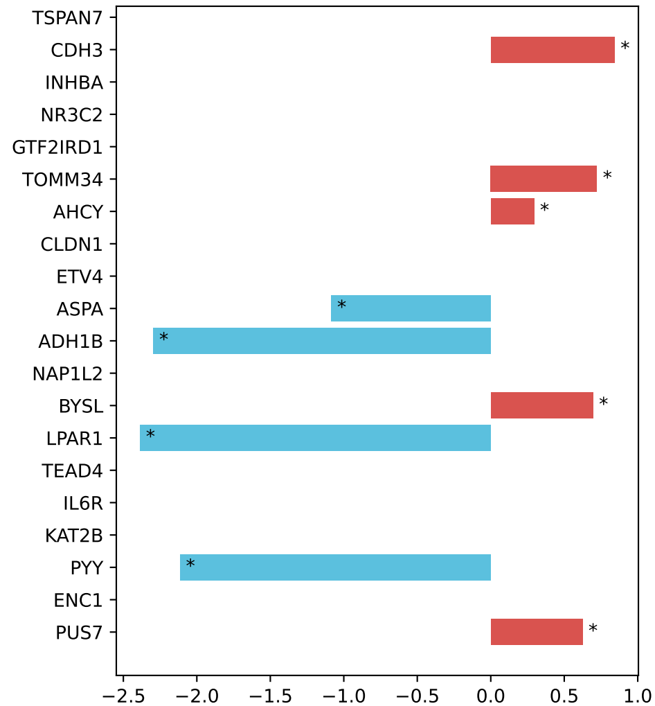
Proteomics Delta Protein (* = Concordant & q<0.05)
