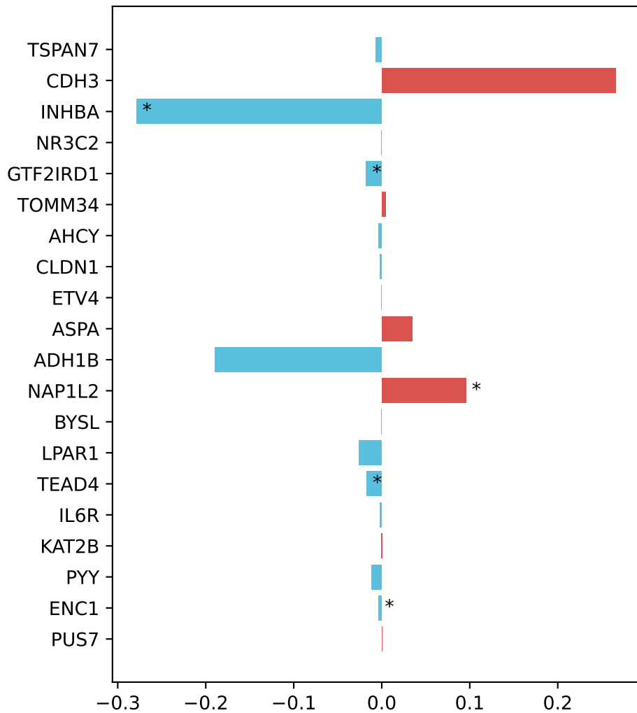
Methylation Delta Beta (* = Concordant & q<0.05)
