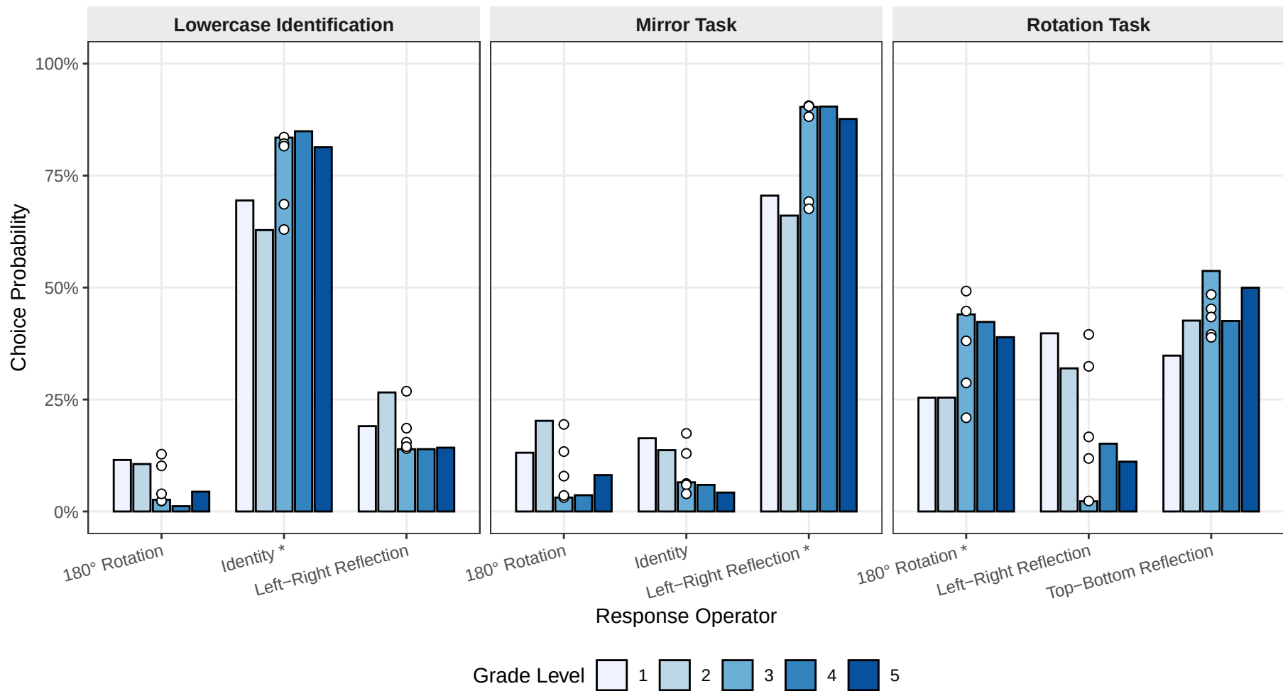
Observed and categorical-model-estimated operator probabilities across grades
