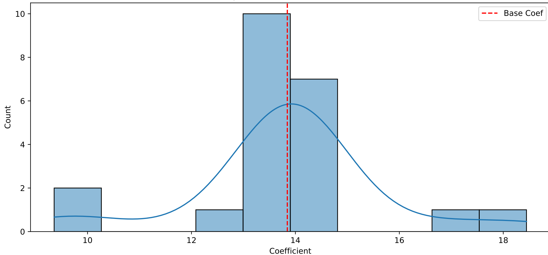
Leave-One-Out Subject Influence on Power vs Dwell Coefficient
