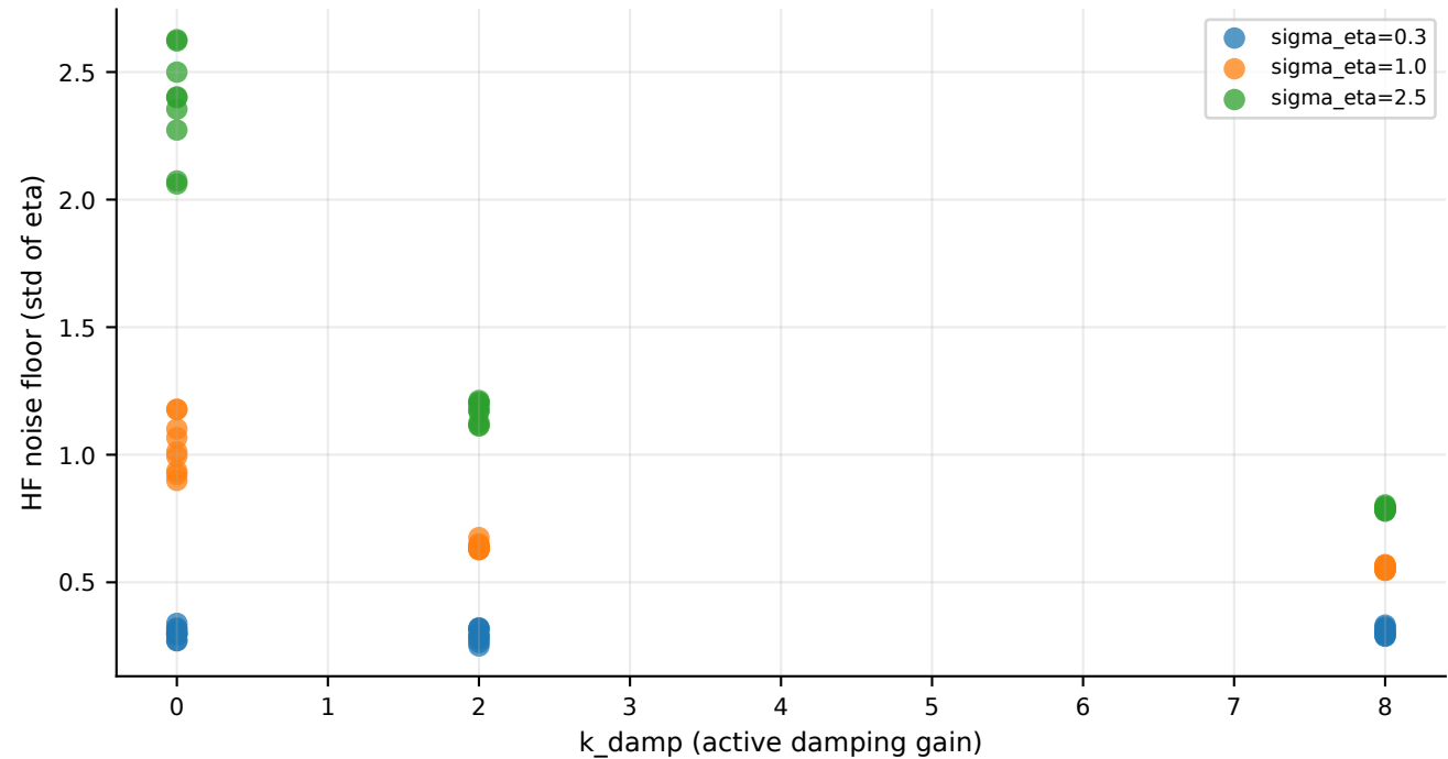
NCTRL2: Active damping vs high-frequency noise floor
