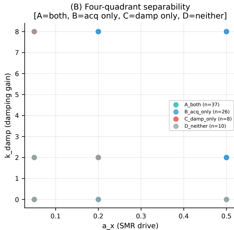
NCTRL8 Figure 2: Separability simulation
