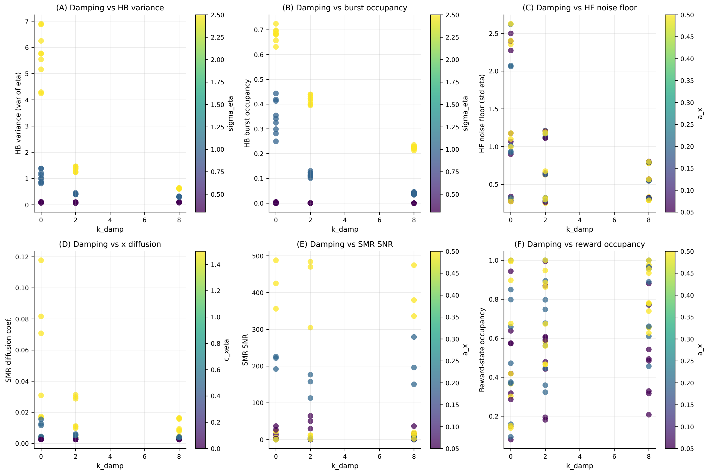
NCTRL8 Figure 3: Noise-control metrics vs damping gain
