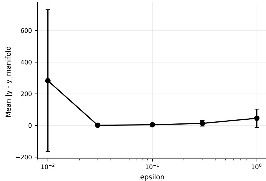
Manifold approximation error vs epsilon
