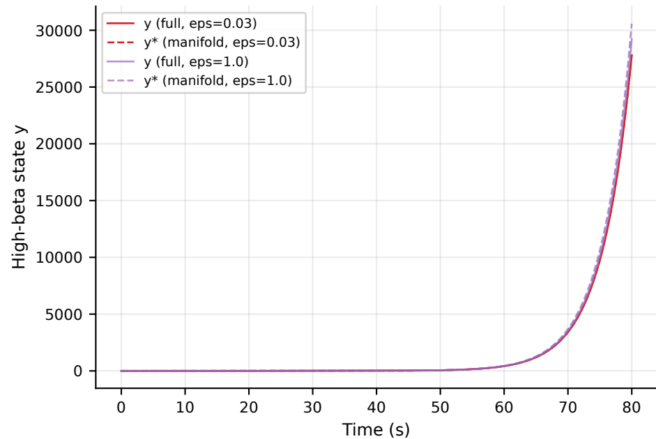
Manifold tracking: fast vs slow epsilon
