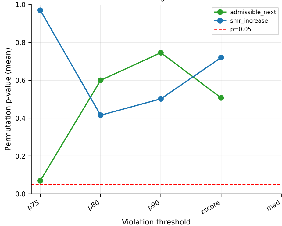
Prediction significance
