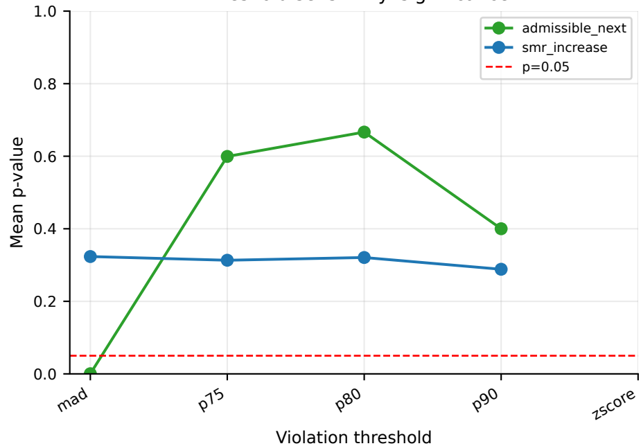
Threshold sensitivity: significance
