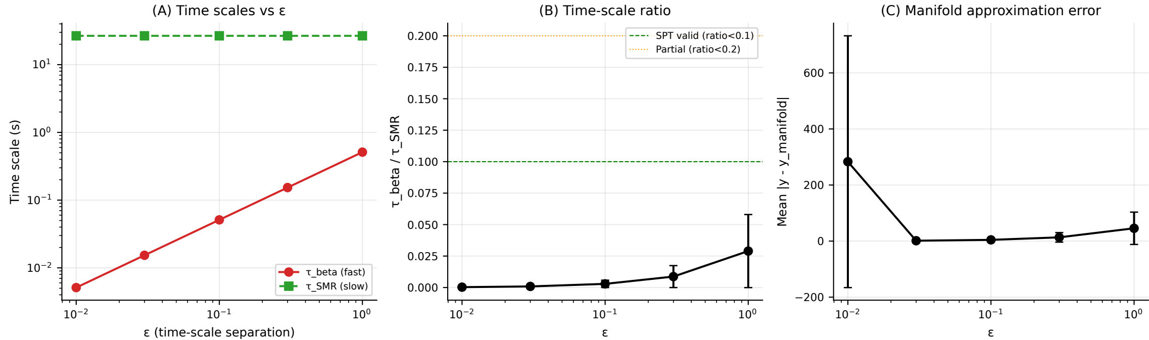
Figure 3: Singular perturbation validity - time-scale separation
