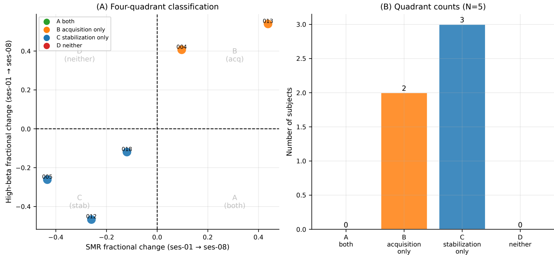
Figure 4: Empirical four-quadrant separability test (N=5 subjects)
