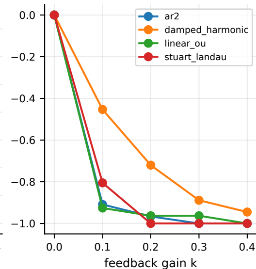
Burst-rate change
