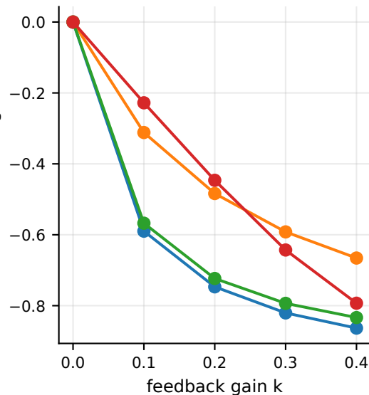
High-beta suppression
