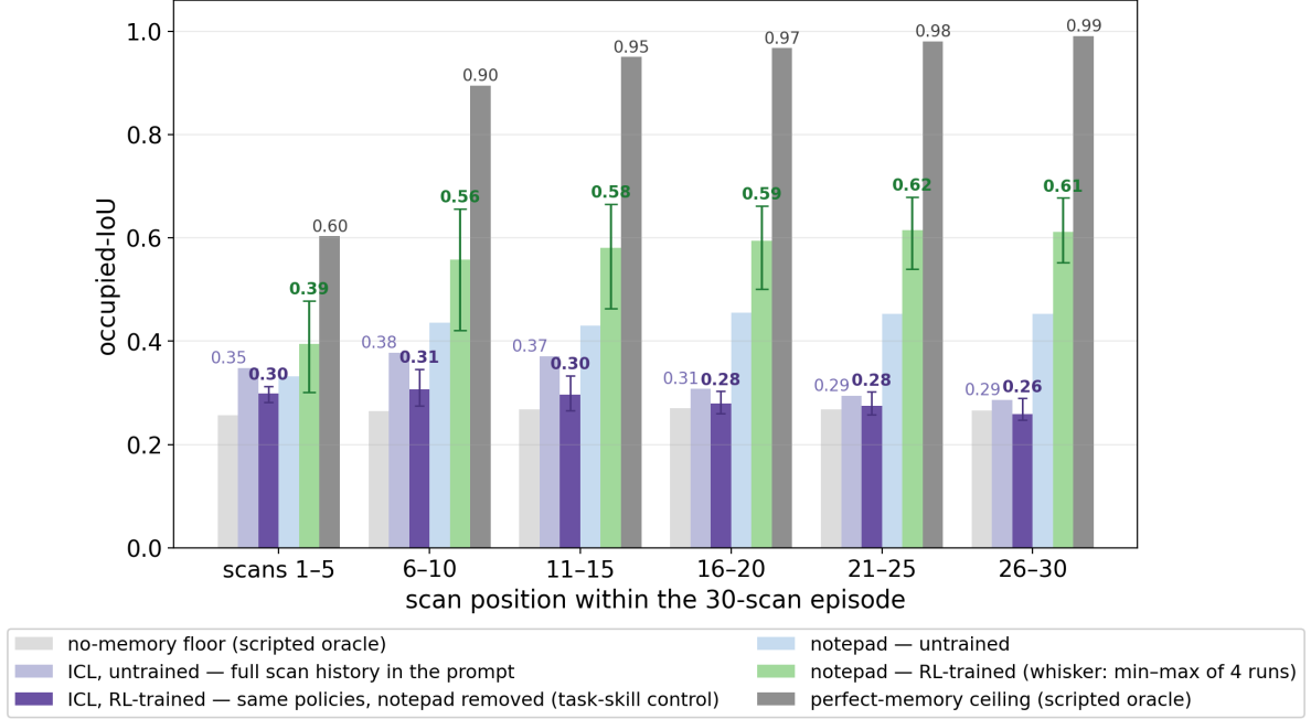
Figure 1: Occupied-IoU by scan position within the 30-scan episode, for the six conditions. Full-history ICL (light purple) peaks at scans 6–10 and then degrades as the transcript grows, ending barely above the scripted no-memory floor (light grey). The untrained notepad (light blue) surpasses ICL from scan 6 onward; RL (green; whiskers give the min–max of the four replicate runs) lifts late-episode accuracy to \approx 0.61 . The ICL-replay control (dark purple) evaluates the same four trained policies with the notepad removed and the full history in the prompt: they score at or below the untrained ICL baseline in every bin and end at the no-memory floor, so the trained gain does not transfer to the task itself. The scripted perfect-memory ceiling (dark grey) rises from 0.60 to 0.99 as the episode uncovers the band.
