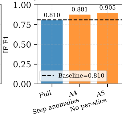
(e) IF F1 (lower = harder to detect)
