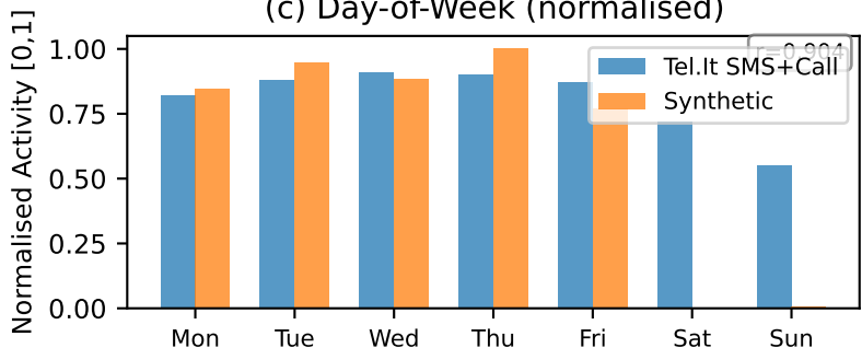
(c) Day-of-Week (normalised)
