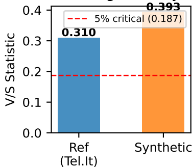
(f) V/S Long-Memory Test
