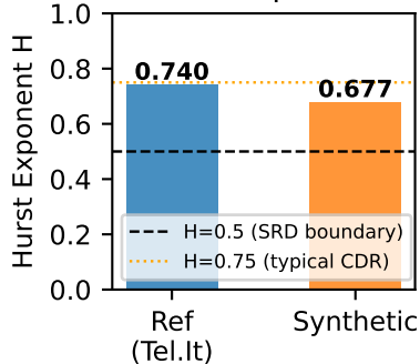
(e) Hurst Exponent R/S
