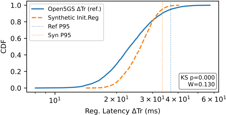
(a) Registration Latency CDF
