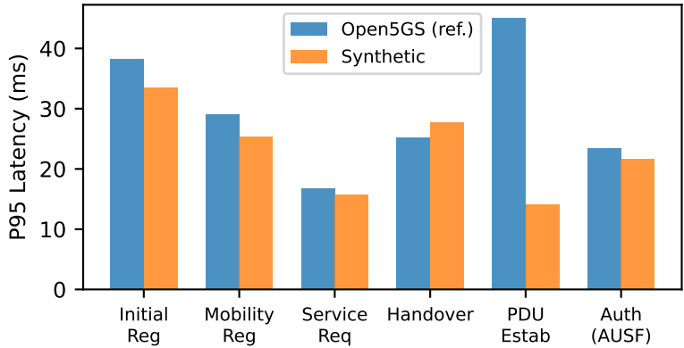
(c) Per-Procedure P95 Latency
