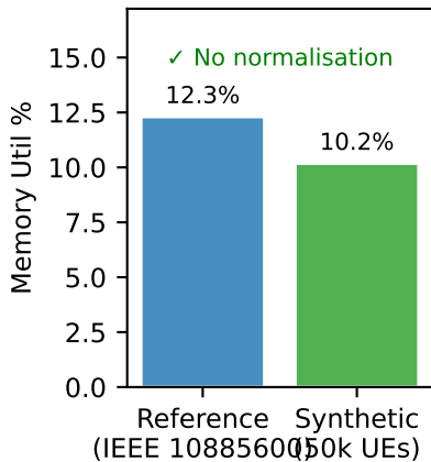
(c) Memory @ 50k UEs Diff=2.1pp
