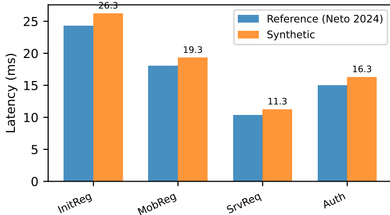
(b) NAS Latency — absolute (ms)
