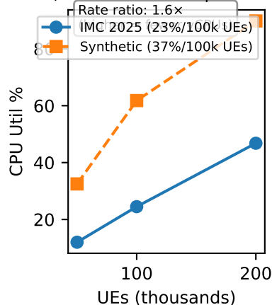
(e) CPU Scaling Rate (rate is vCPU-independent)
