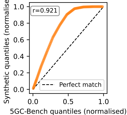
(b) Q-Q: CPU Scaling
