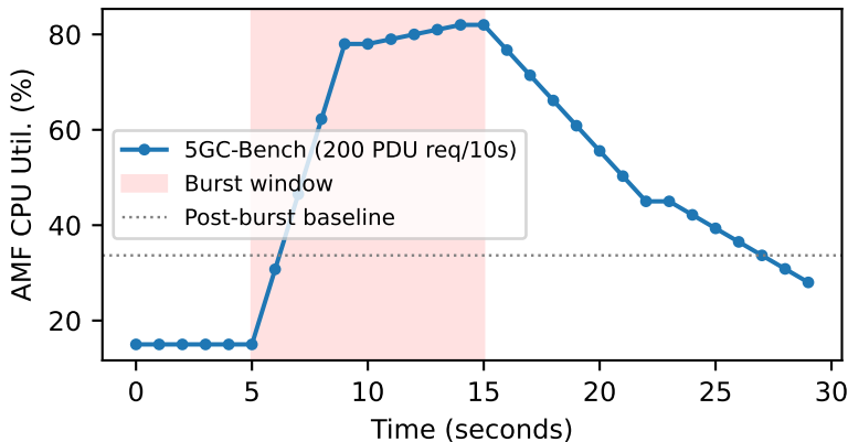
(c) PDU Session Burst Recovery Profile
