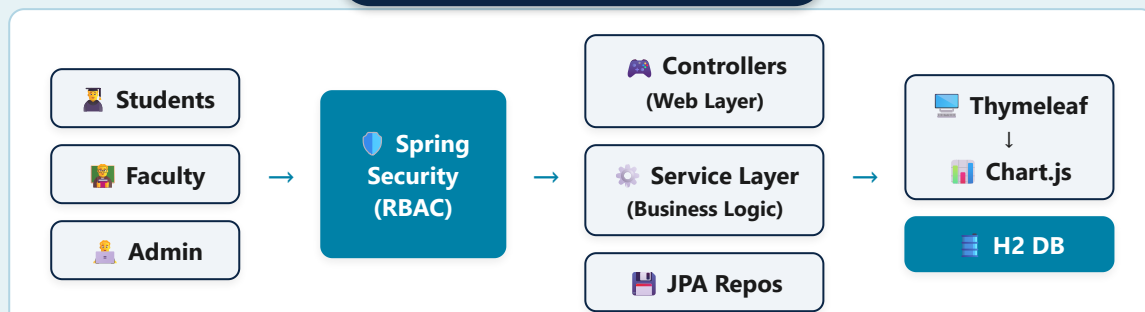
Layered MVC Architecture with Role-Based Security
