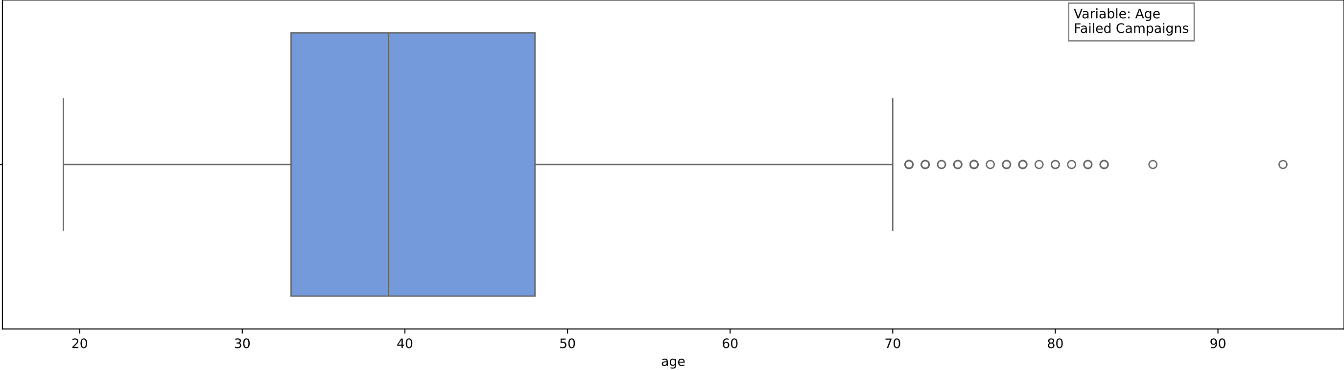
Boxplots of Continuous Variables in Dataset
