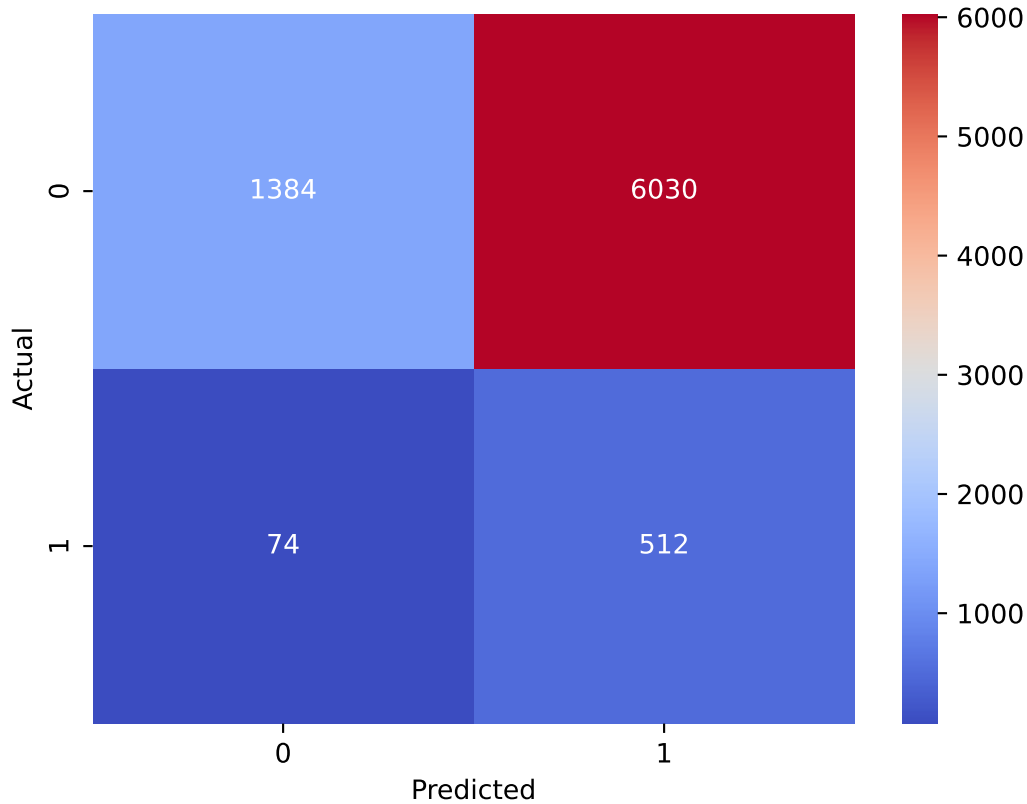
SGDClassifier Confusion Matrix
