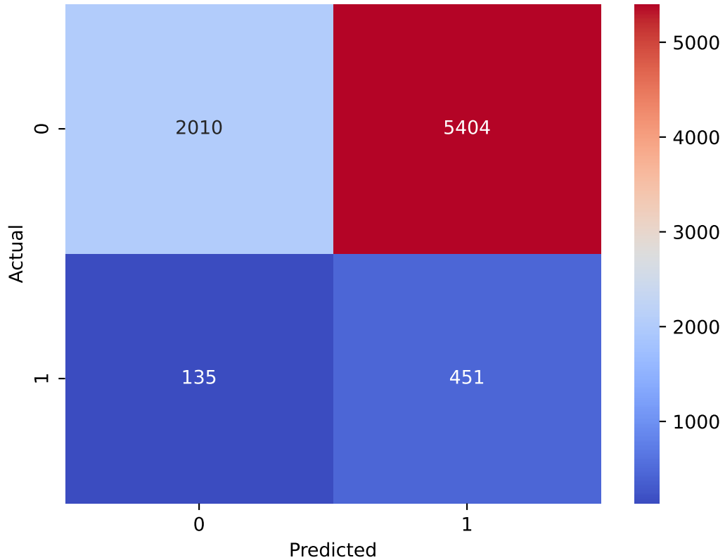
LGBMClassifier Confusion Matrix
