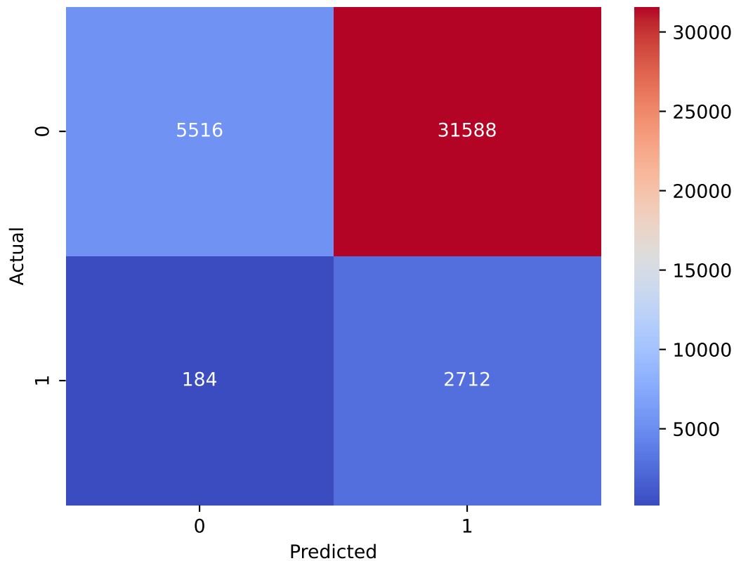
LGBMClassifier Confusion Matrix on Full Dataset
