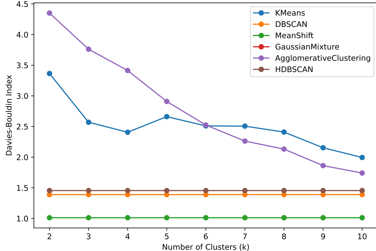
Davies-Bouldin Index vs. Number of Clusters
