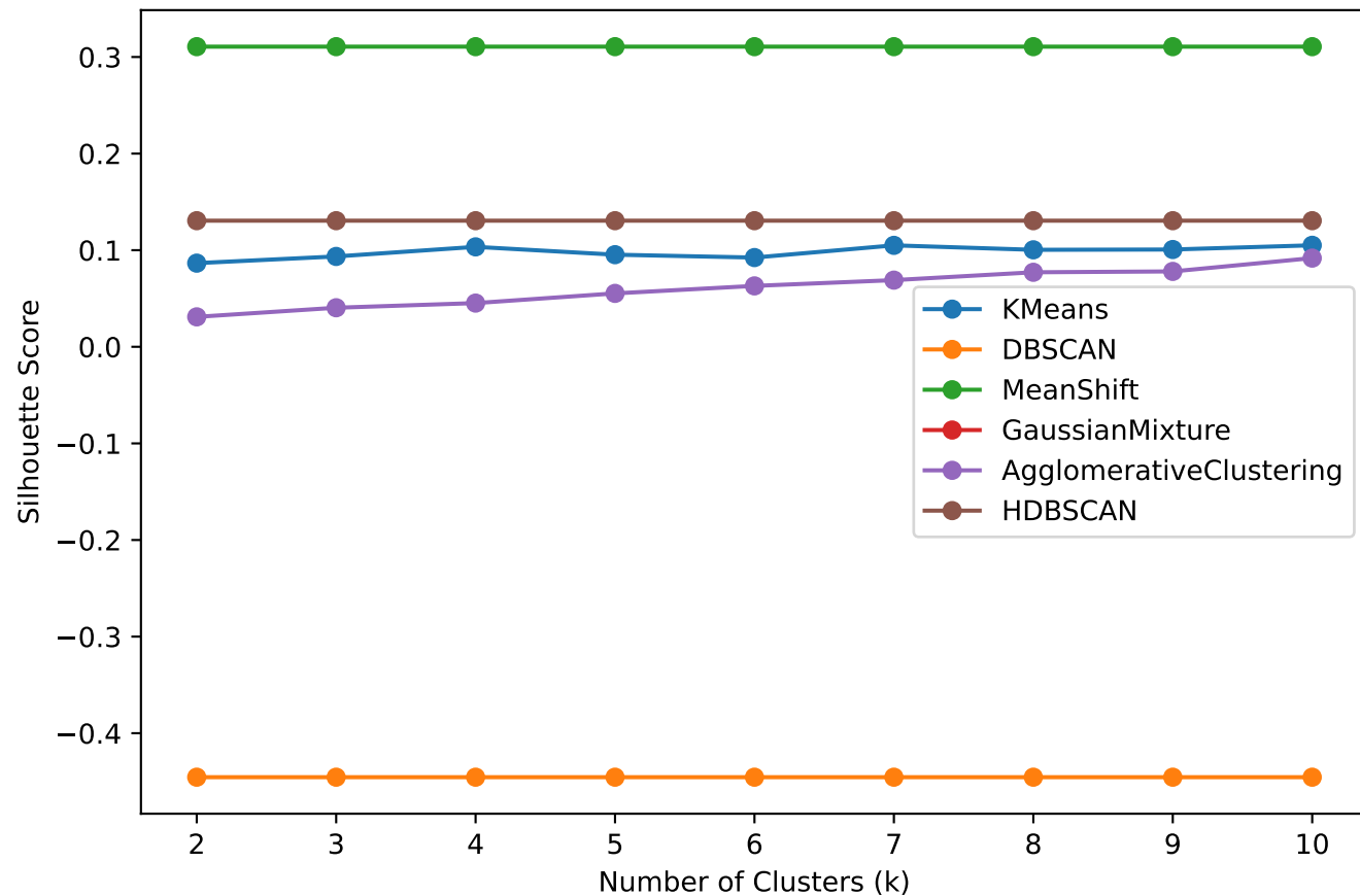
Silhouette Score vs. Number of Clusters
