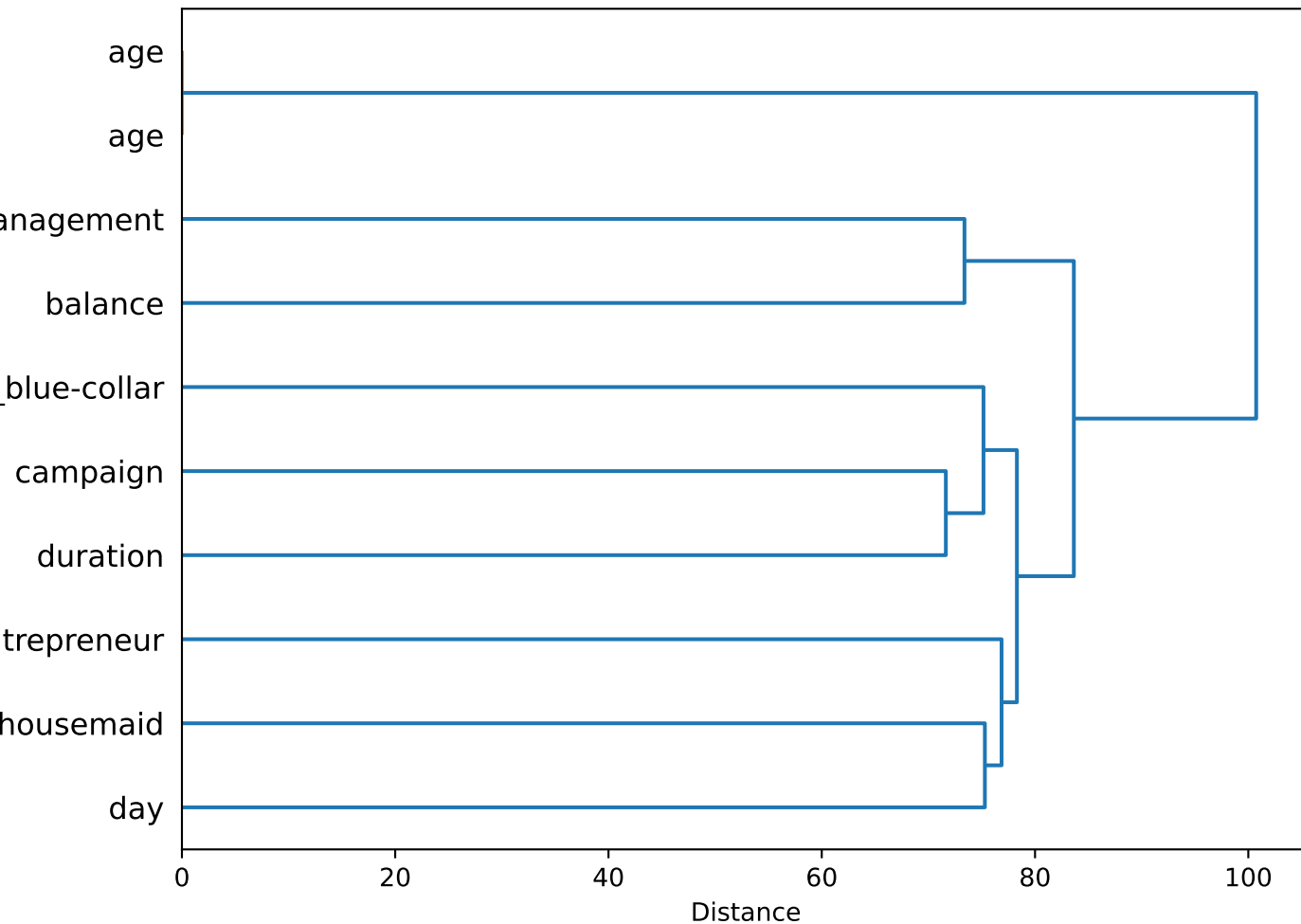
Dendrogram of Top Feature Linkages
