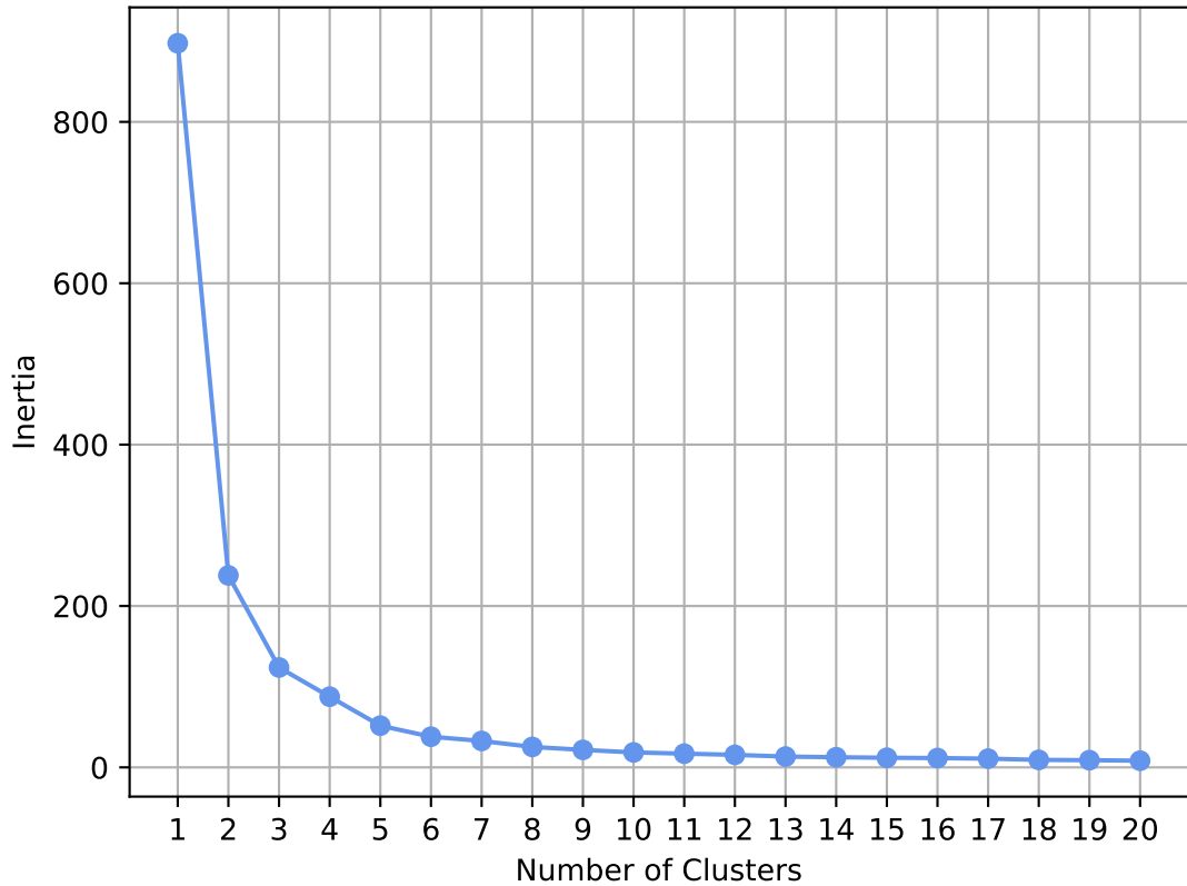
Elbow Plot for Optimal Number of Clusters
