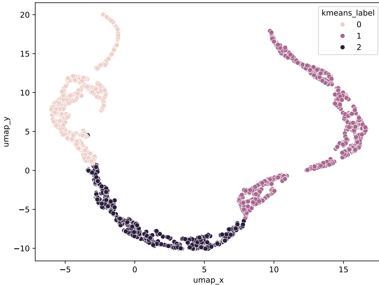
UMAP 2D Projection
